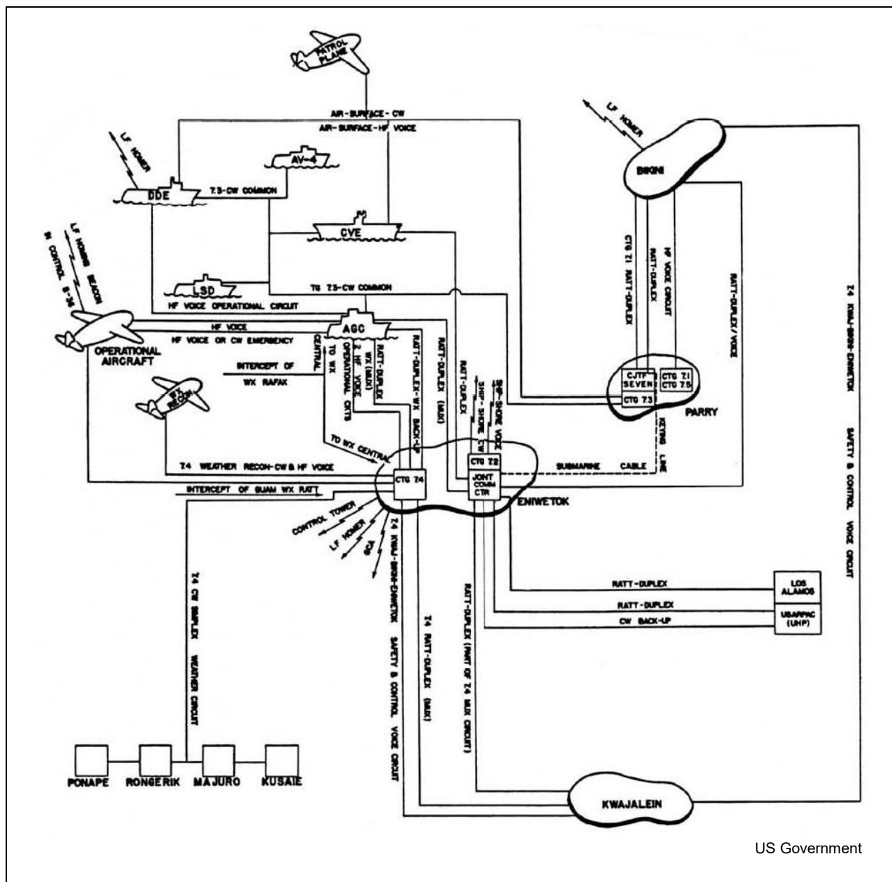
Figure 5-3. Principal task force HF radio circuits The task force command ship USS Estes was the “AGC” shown toward the center of the diagram. The square labeled “CTG 7.4” on Eniwetok was the Airways and Air Communications Service Center; the “CTG 7.2” square on Eniwetok was the Army Communications Service Center. Reproduced from Appendix I to Annex E of Operation Plan No. 1-53 (J-22100 [1953]). Radio communications could be difficult with the Weather Island service detachments, including the unit at Rongerik. “The location of the Weather Central antenna was found to be too close to the Air Operations Center (AOC) and Combat Information Center (CIC) receiving circuit, causing garbled reception. An investigation into the situation revealed no practical solution other than eliminate, as much as possible, conversation between the AOC and CIC during the time weather information is being received.” (NV0076407, 12)
