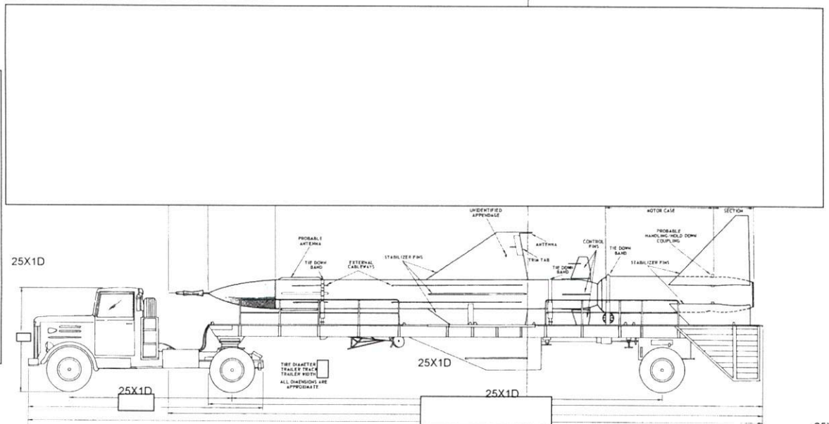
FIGURE 6. DIMENSIONAL DRAWINGS OF MISSILE AND TRACTOR-TRAILER.
