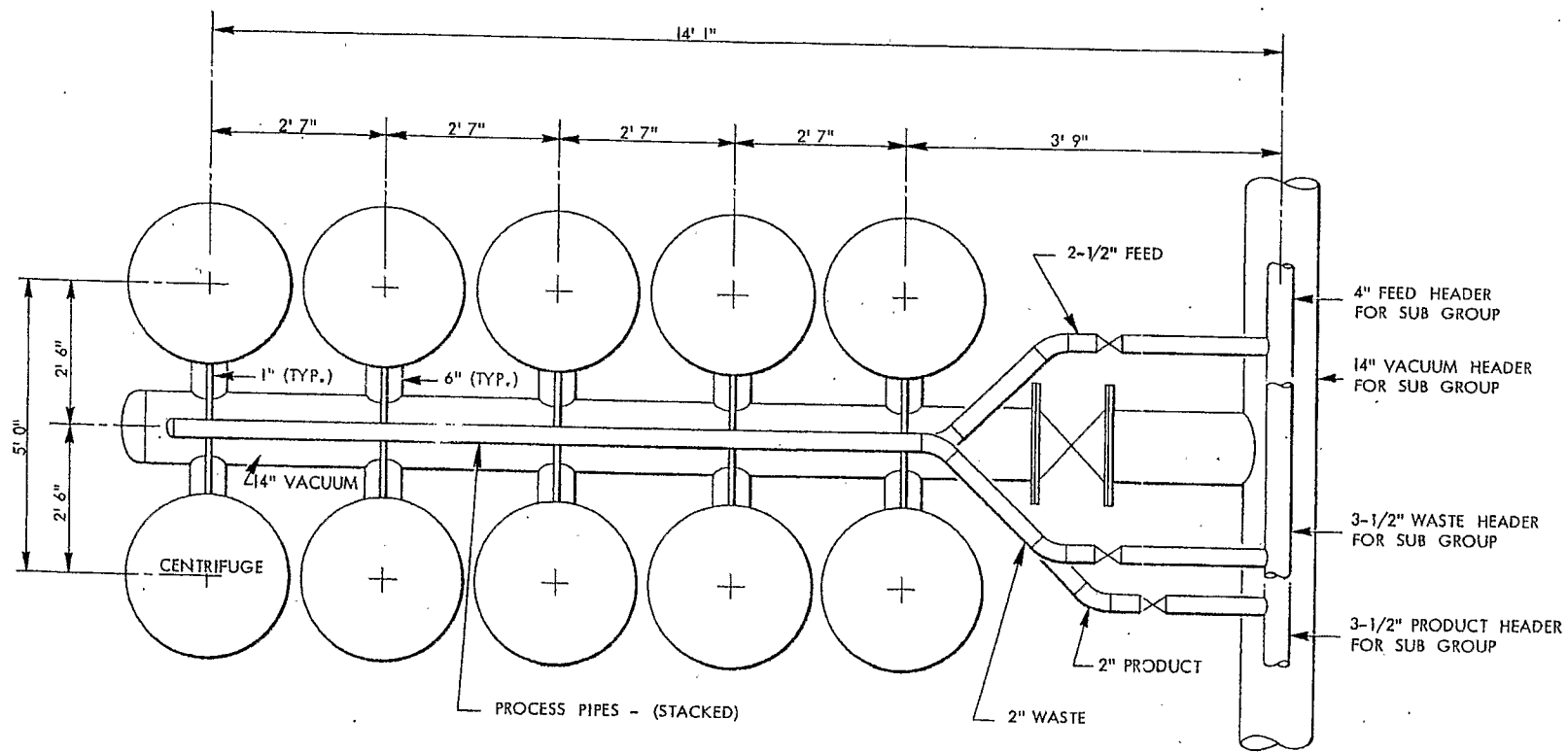
Figure 5 10-CENTRIFUGE PARALLEL CELL
