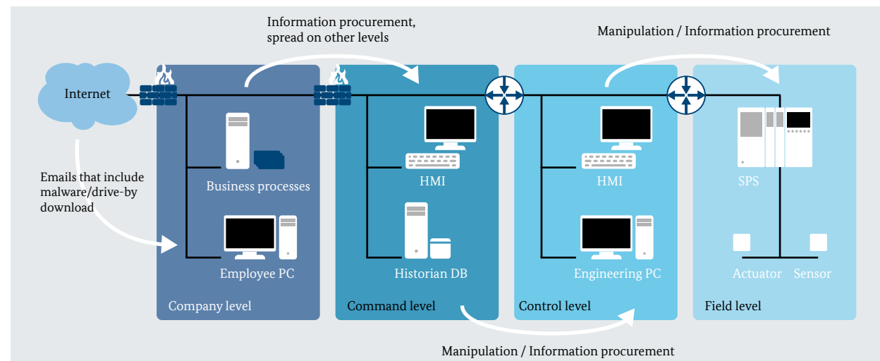
Figure 3: The process of multi-staged attacks on a typical ICS infrastructure
