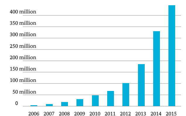
Figure 4: Number of known versions of malicious programs for Windows
