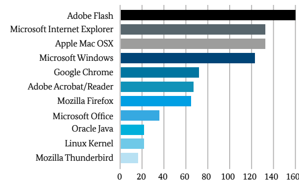
Figure 2: Critical vulnerabilities of the software products logged in the BSI vulnerability traffic light system by September 2015
