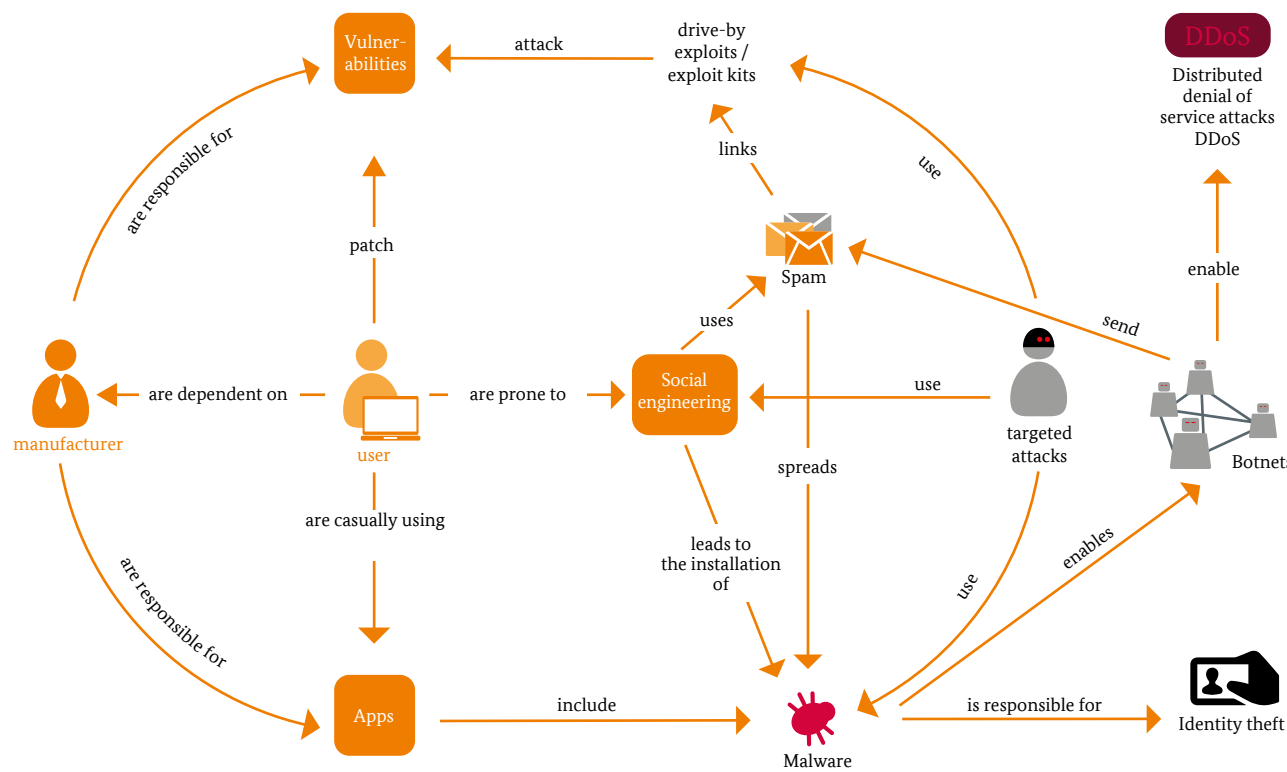
Figure 14: Causes of current security threats
