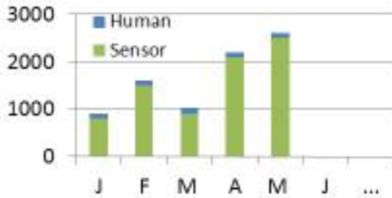
Attack Techniques
